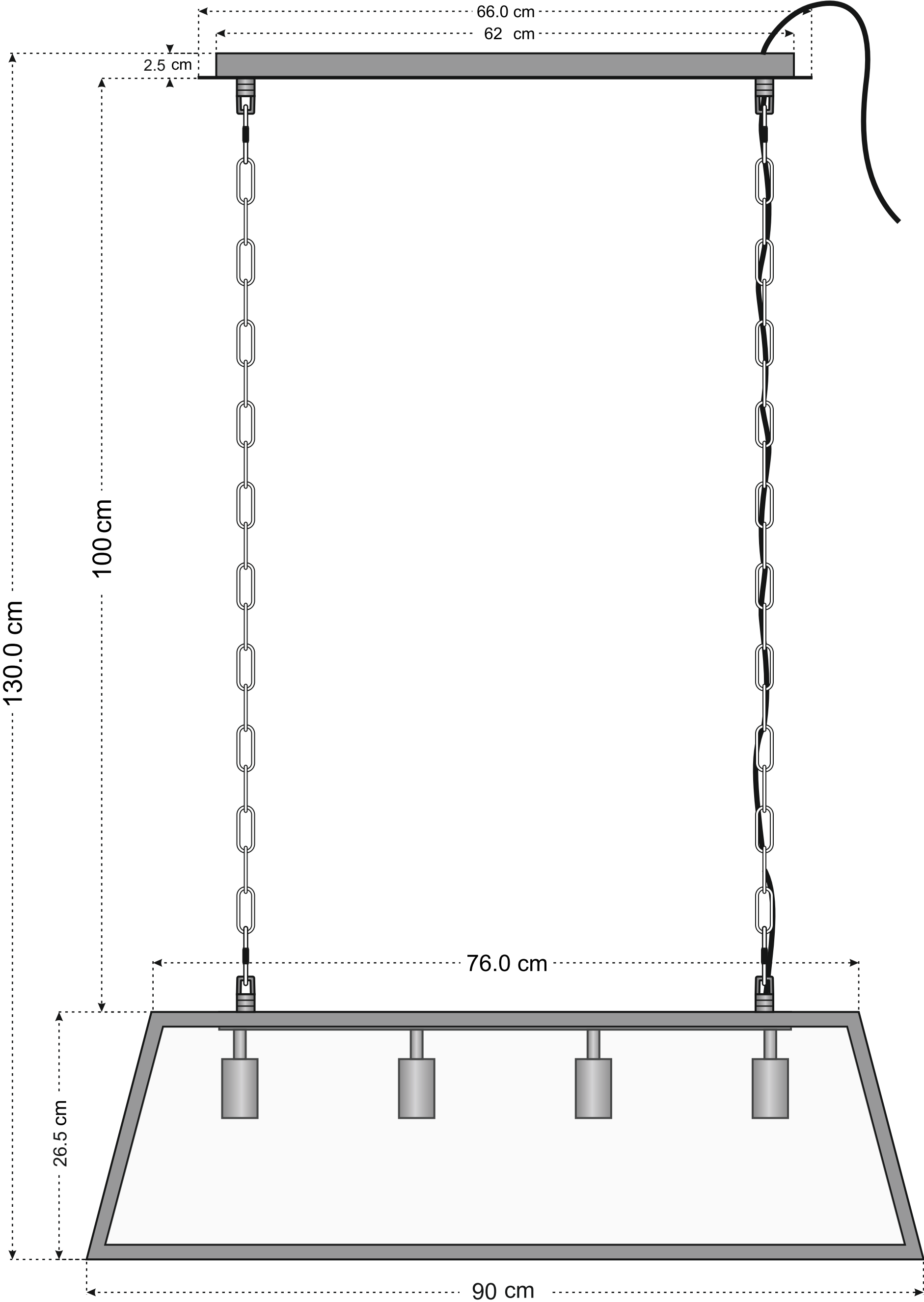
Front View
